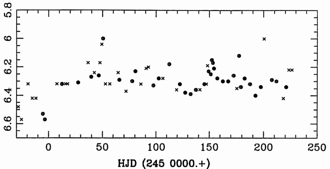
Fig. 2. 1995-96 GEOS visual observations of OT Gem. Crosses are single observations while the solid circles are averages of nearby multiple observations as described in the text.
