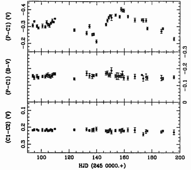
Fig. 1. 1996 observations of OT Gem carried out at La Luz Observatory. The top panel displays OT Gem (P) - HR2780 (C1) light variations in Johnson's V filter. The medium panel shows the same in B-V. The bottom panel shows HR2780 (C1) - HR2858 (C2) in V filter.
