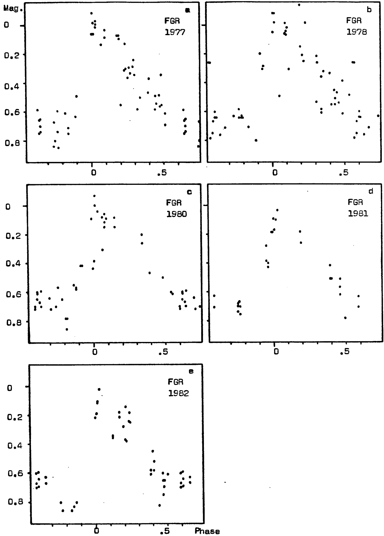
Fig. 4. Combined light curves of V 514 Cyg.
